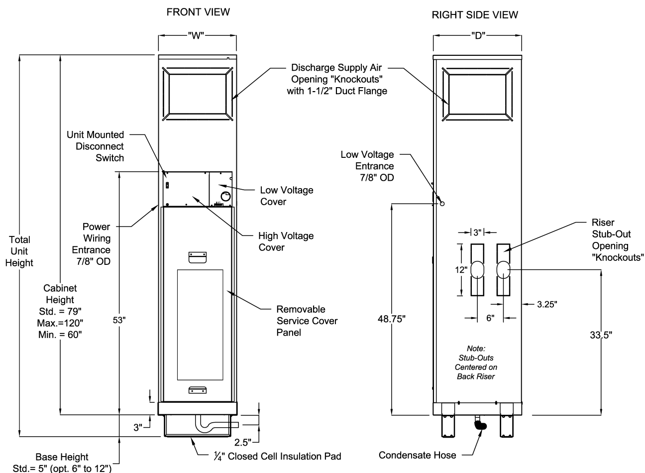
VSHY Cabinet Dimensions (Silver & Gold Series)
