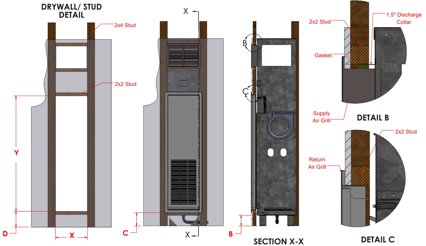
Acoustic Panel Furring Detail—Front & Side View
